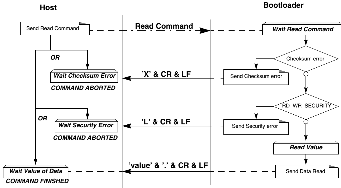
Figure 24-16. Read Flow
