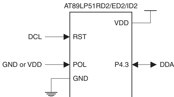
Figure 23-1. AT89LP51RD2/ED2/ID2 On-Chip Debug Connections
