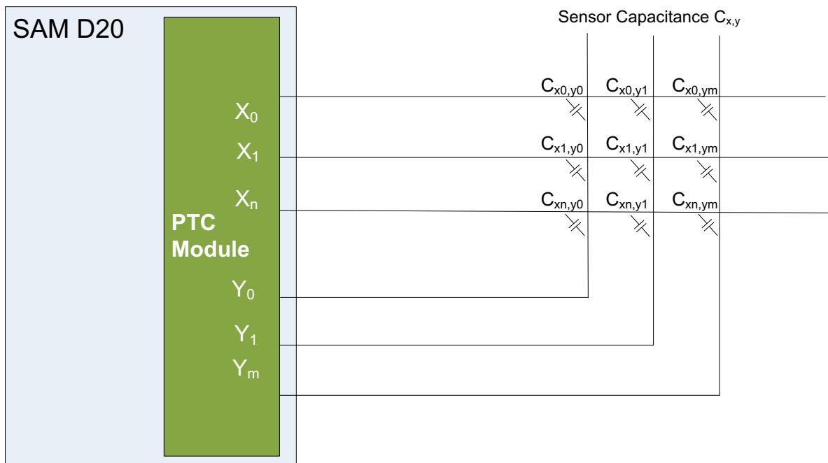
Figure 31-3. Mutual Capacitance Sensor Arrangement
