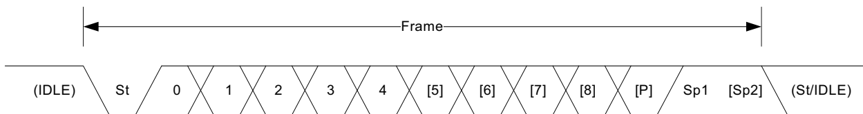
Figure 24-2. Frame Formats
