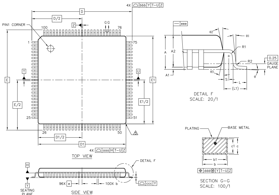
Figure 4.2. LQFP100
