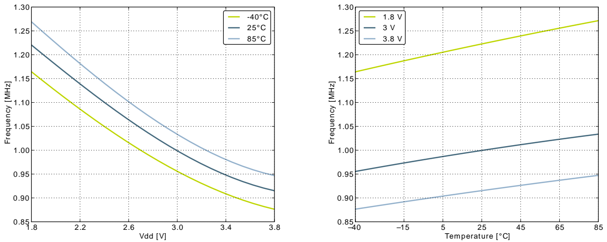
Figure 3.10. Calibrated HFRCO 7 MHz Band Frequency vs Temperature and Supply Voltage
