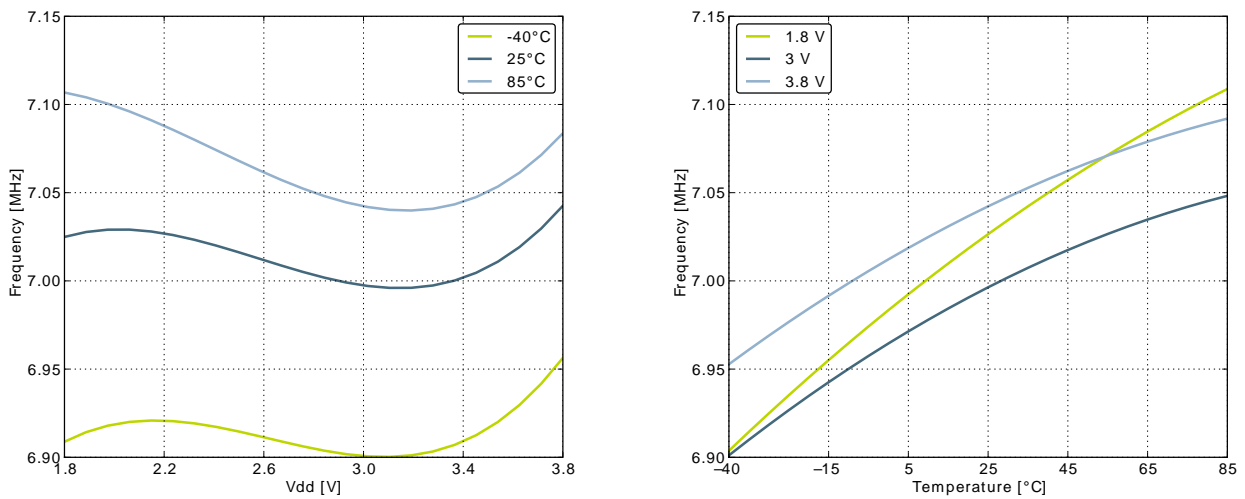
Figure 3.11. Calibrated HFRCO 11 MHz Band Frequency vs Temperature and Supply Voltage
