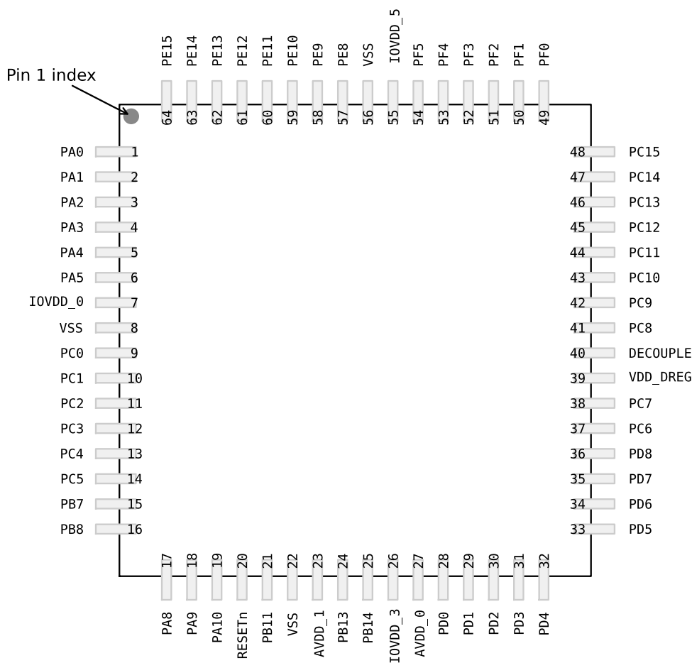
Figure 4.1. EFM32TG232 Pinout (top view, not to scale)
