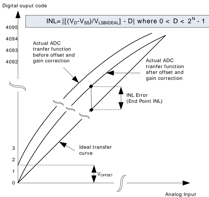
Figure 3.28. Integral Non-Linearity (INL)
