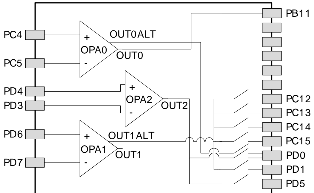
Figure 4.2. Opamp Pinout
