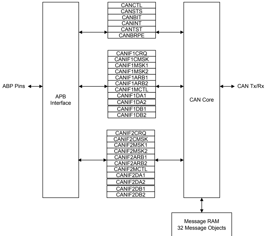
Figure 13-1. CAN Module Block Diagram
