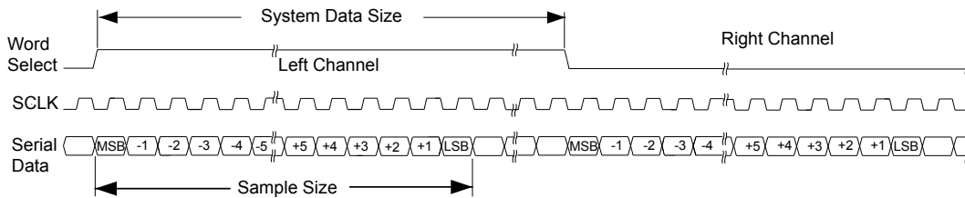
Figure 17-3. Left-Justified Data Transfer
