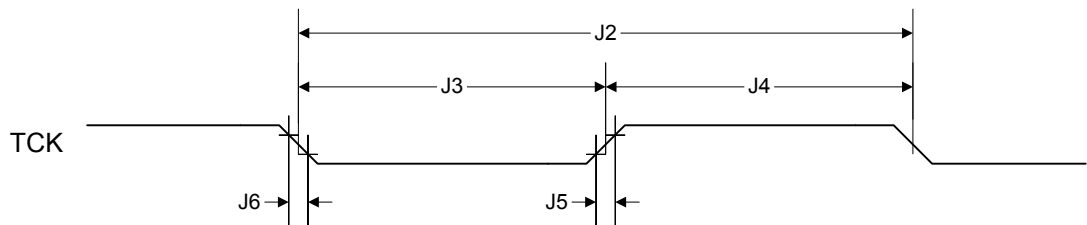
Figure 27-4. JTAG Test Clock Input Timing
