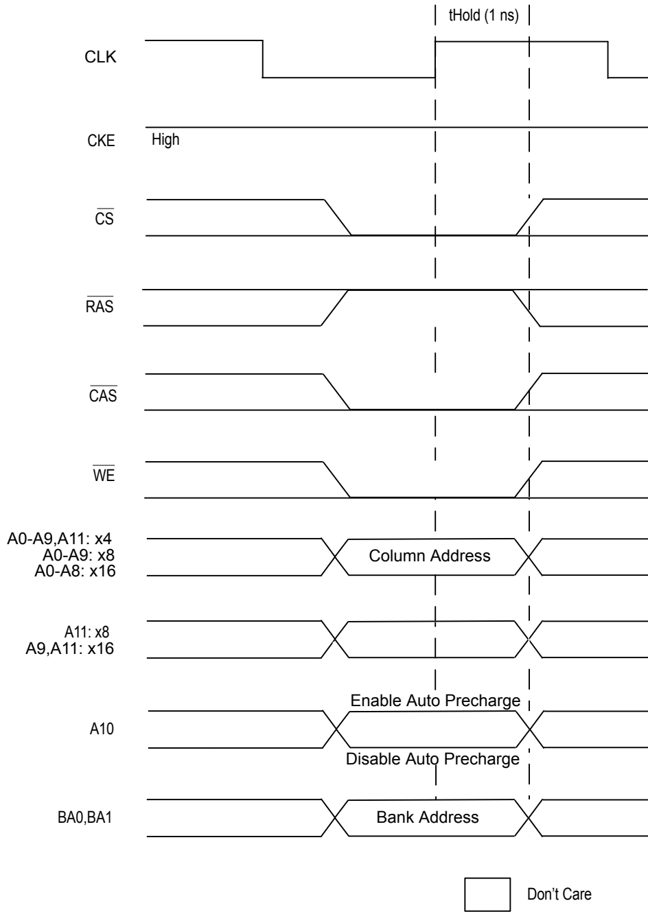
Figure 27-14. SDRAM Write Command Timing
