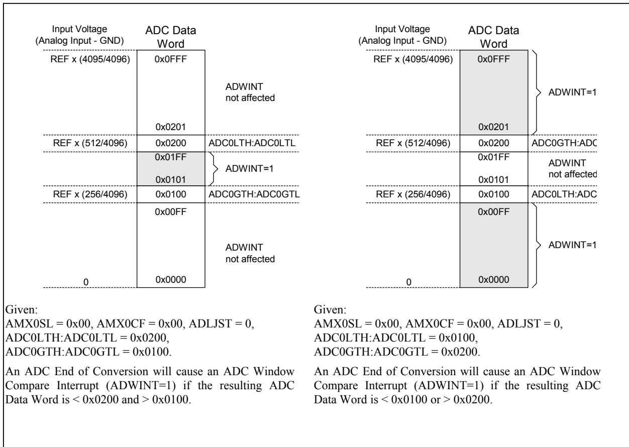
Figure 6.12. 12-Bit ADC Window Interrupt Examples, Right Justified Data
