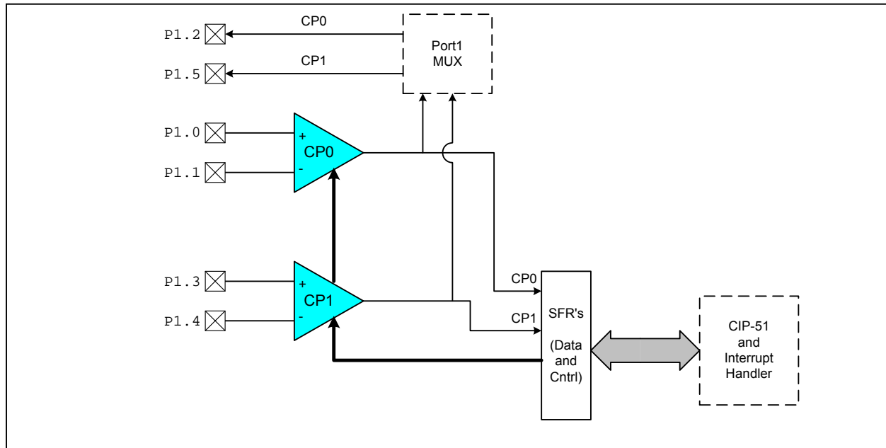
Figure 1.11. Comparator Diagram
