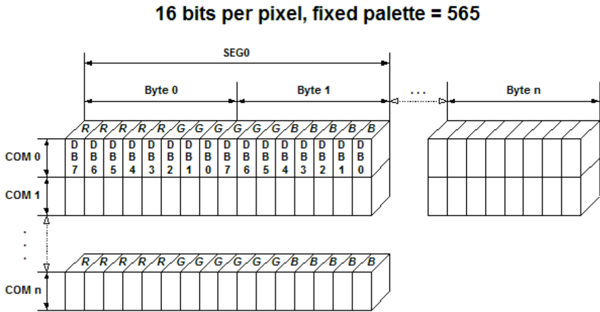
Relationship between memory and the SEG and COM lines for 16bpp mode.
